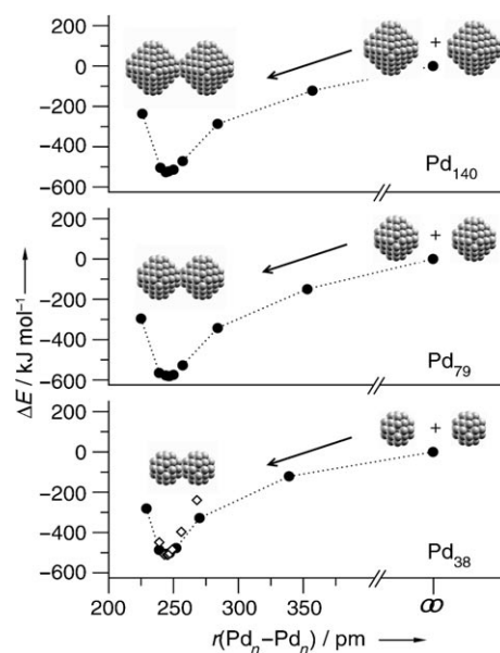
Figure 1. Interaction energy \Delta E(\text{VWN}) of Pd n clusters ( n = 38, 79, 140 ) as a function of the distance r(\text{Pd}_n\text{-Pd}_n) during formation of (Pd n ) x nanowires through the (100) facets for partially (●) and fully optimized (<math>\diamond</math>) interacting clusters. Dotted lines are guides to the eye.
